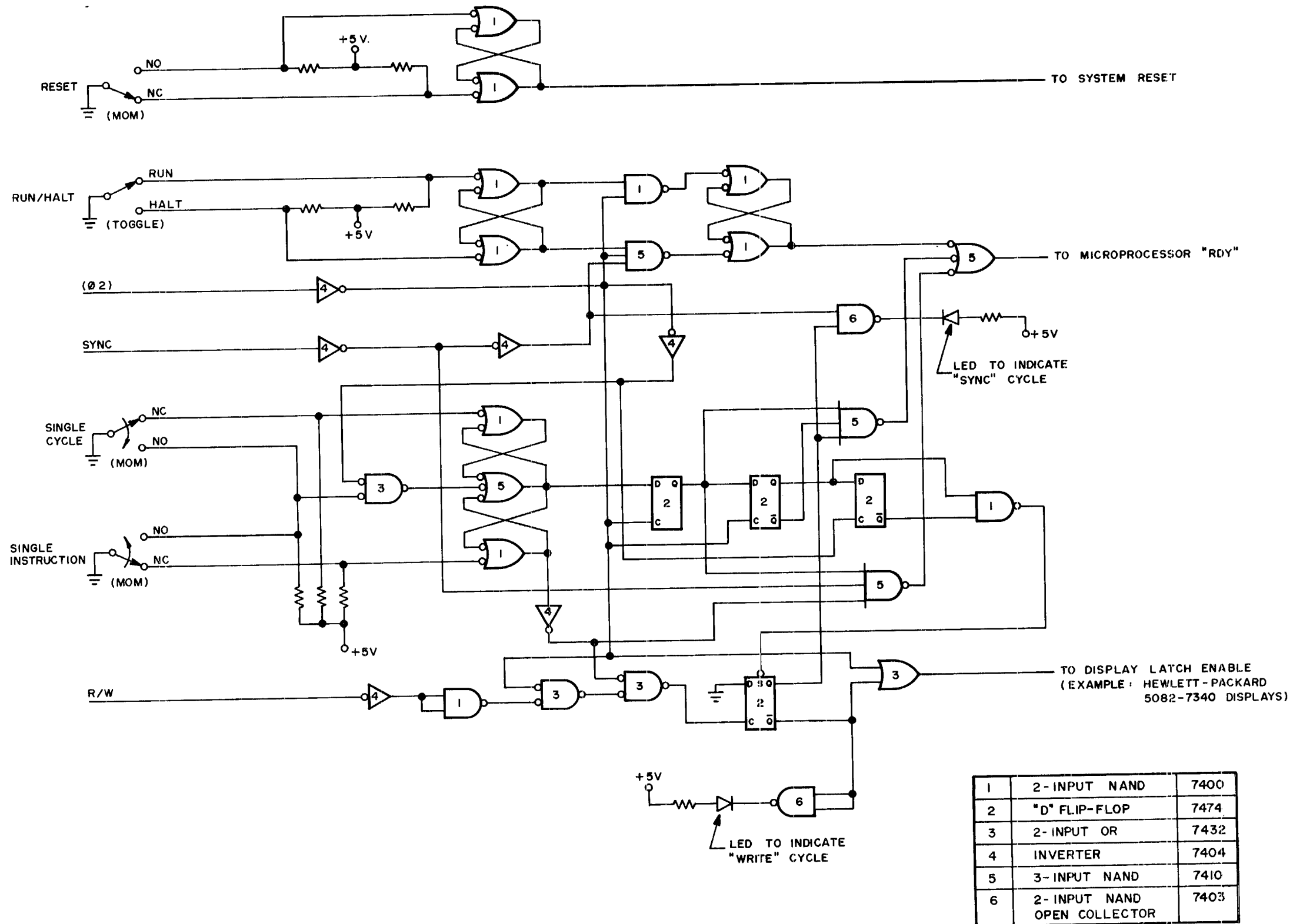
Suggested Static Test Control Logic FIGURE 3.1
